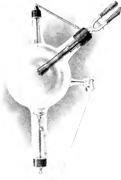
FIG. 27.—Cyclops radiator tube. (C. Andrews.)
